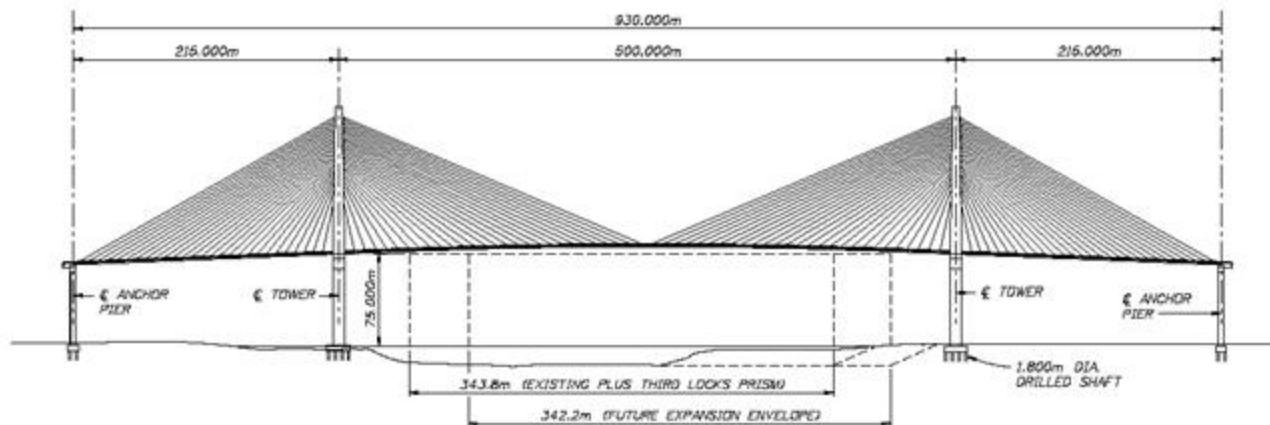
ELEVATION VIEW
